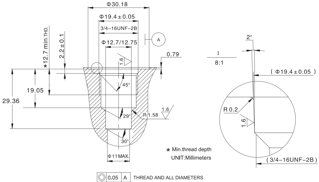
CAVITY:08W-2
