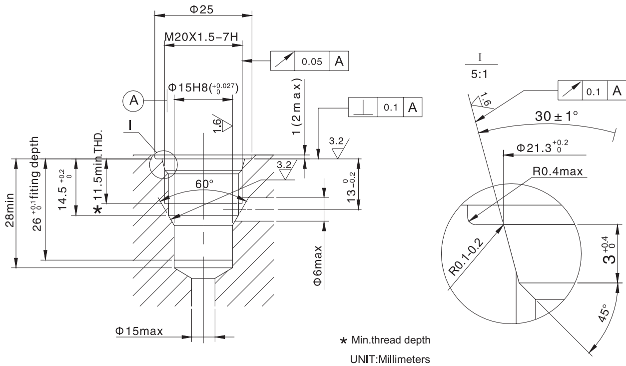
CAVITY:HYDAC 06020
